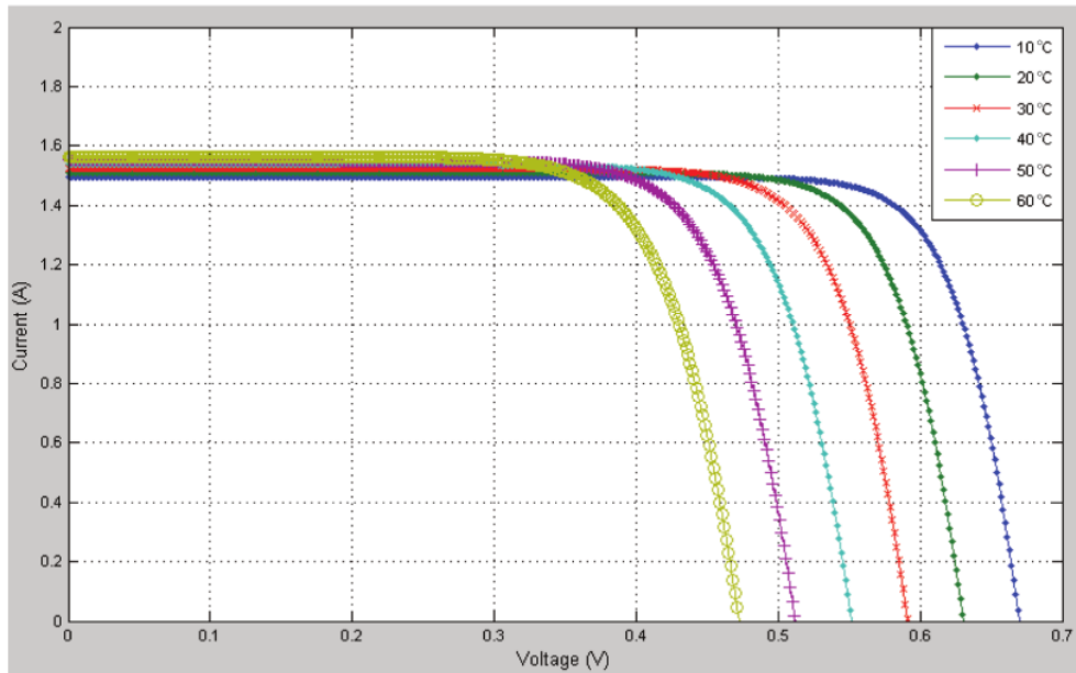
(b) Constant irradiance of 800 W/m 2
