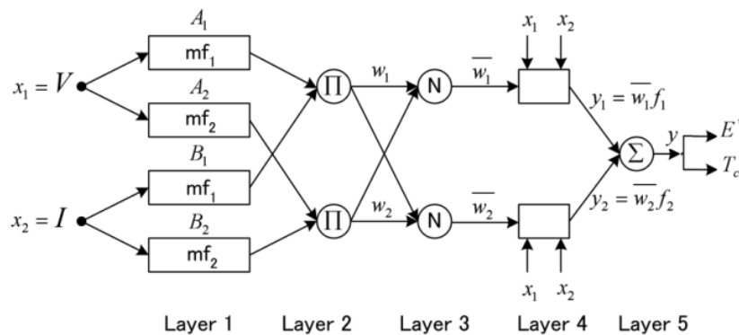
FIGURE 4. ANFIS structure for the first-order Sugeno type
