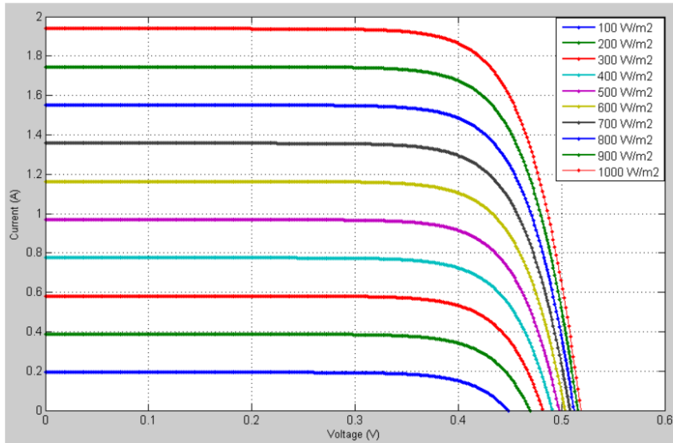
(a) Constant temperature of 50°C
