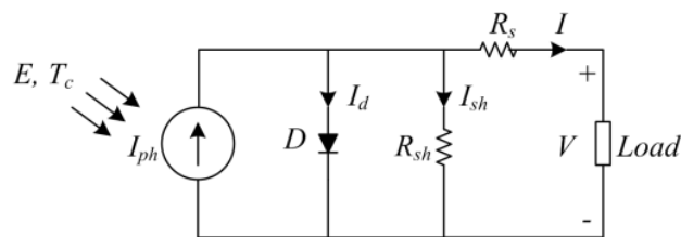
FIGURE 2. Electric circuit of modeling of solar cell
