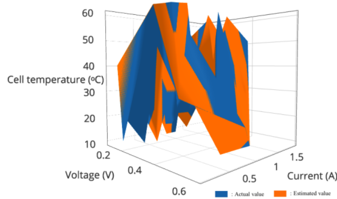
(b) Cell temperature
